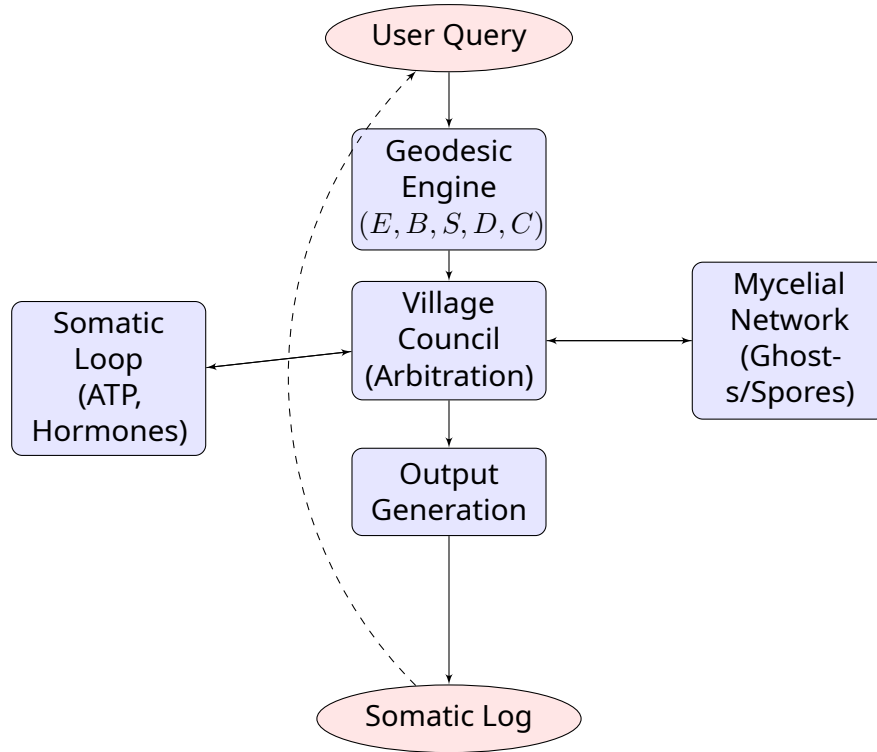
Figure 1: System Architecture: The flow of information from Geodesic projection through Village arbitration and Metabolic costing. Note the feedback loop returning somatic data to the user.
